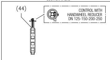
SUCTION VALVE
