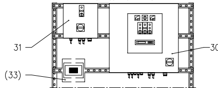
PUMP CONTROL PANELS
