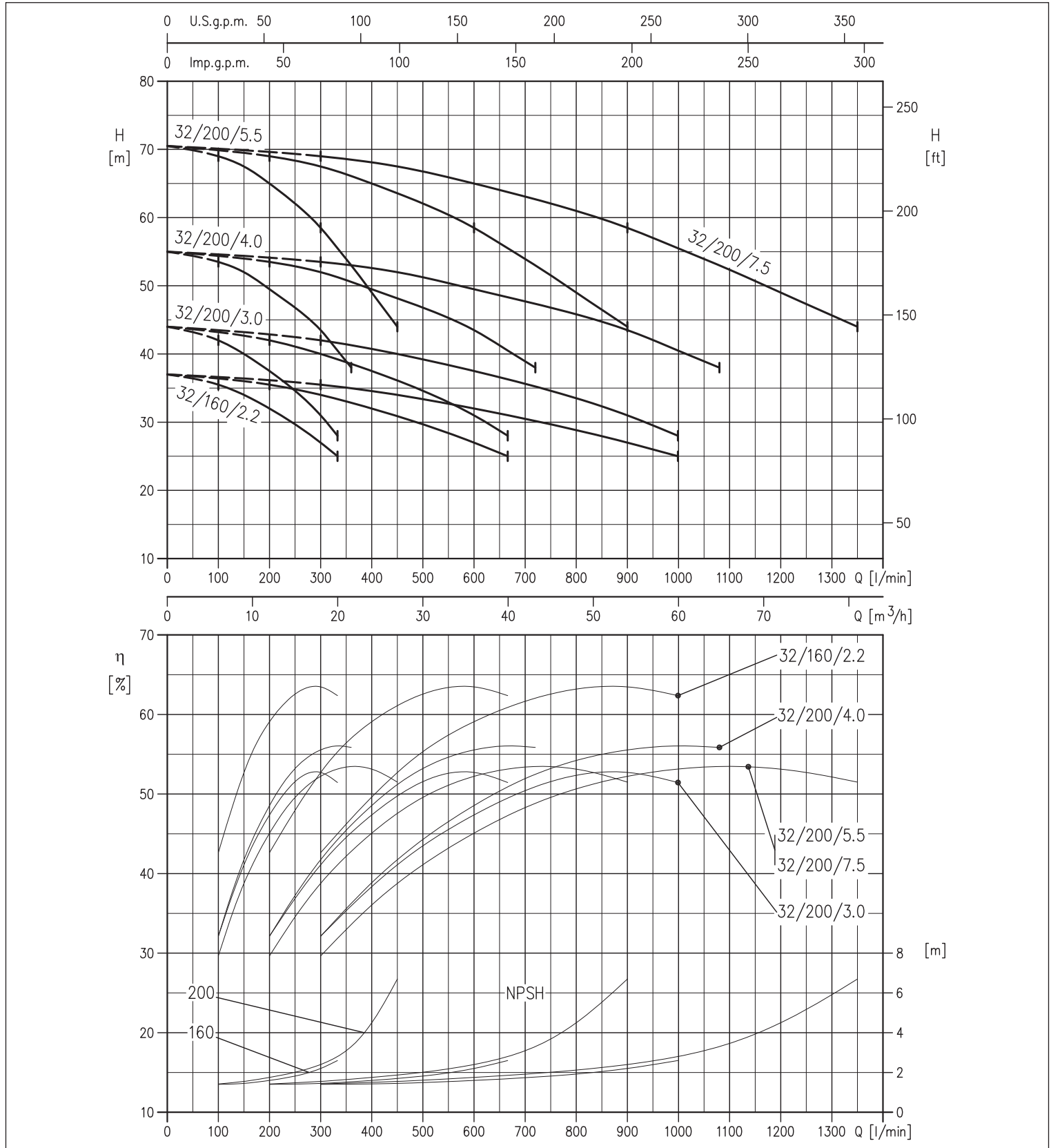
3GP 3M 32 RANGE PERFORMANCE CURVE (according to ISO 9906 Attachment A)
