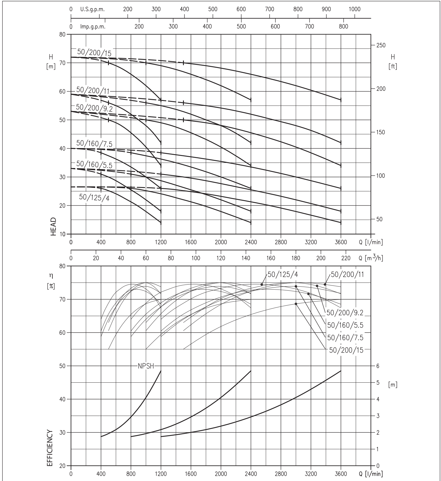
3GP 3M 50 RANGE PERFORMANCE CURVE (according to ISO 9906 Attachment A)
